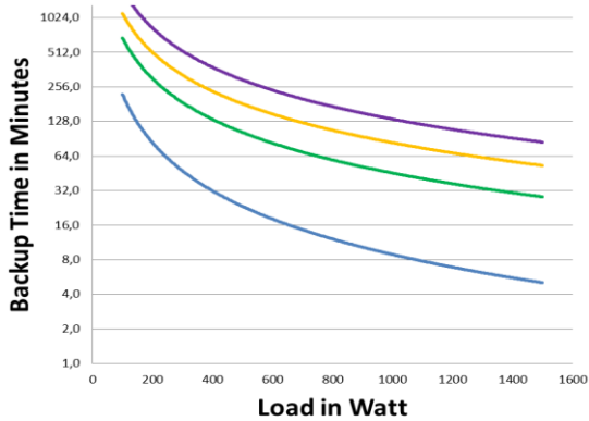
PowerWalker VI 2000RT LCD
